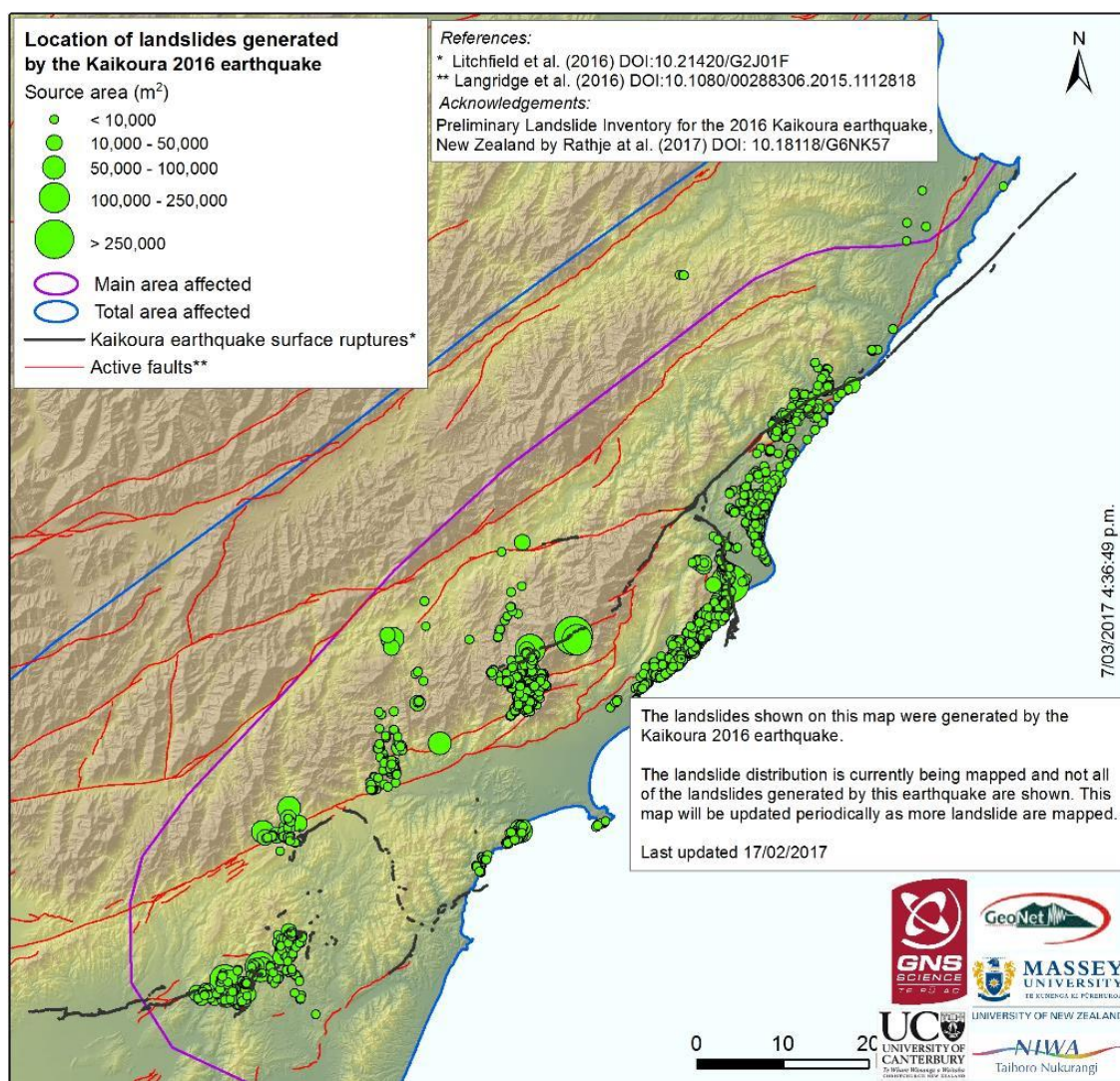
Figure 9: The landslide inventory for the 14 November 2016 M_w 7.8 Kaikōura earthquake as at 17 February 2017 (estimate 30% complete). The active fault ruptures cause by the earthquake are shown as black lines on the map. The landslides, and particularly the largest landslides cluster around the fault ruptures.
